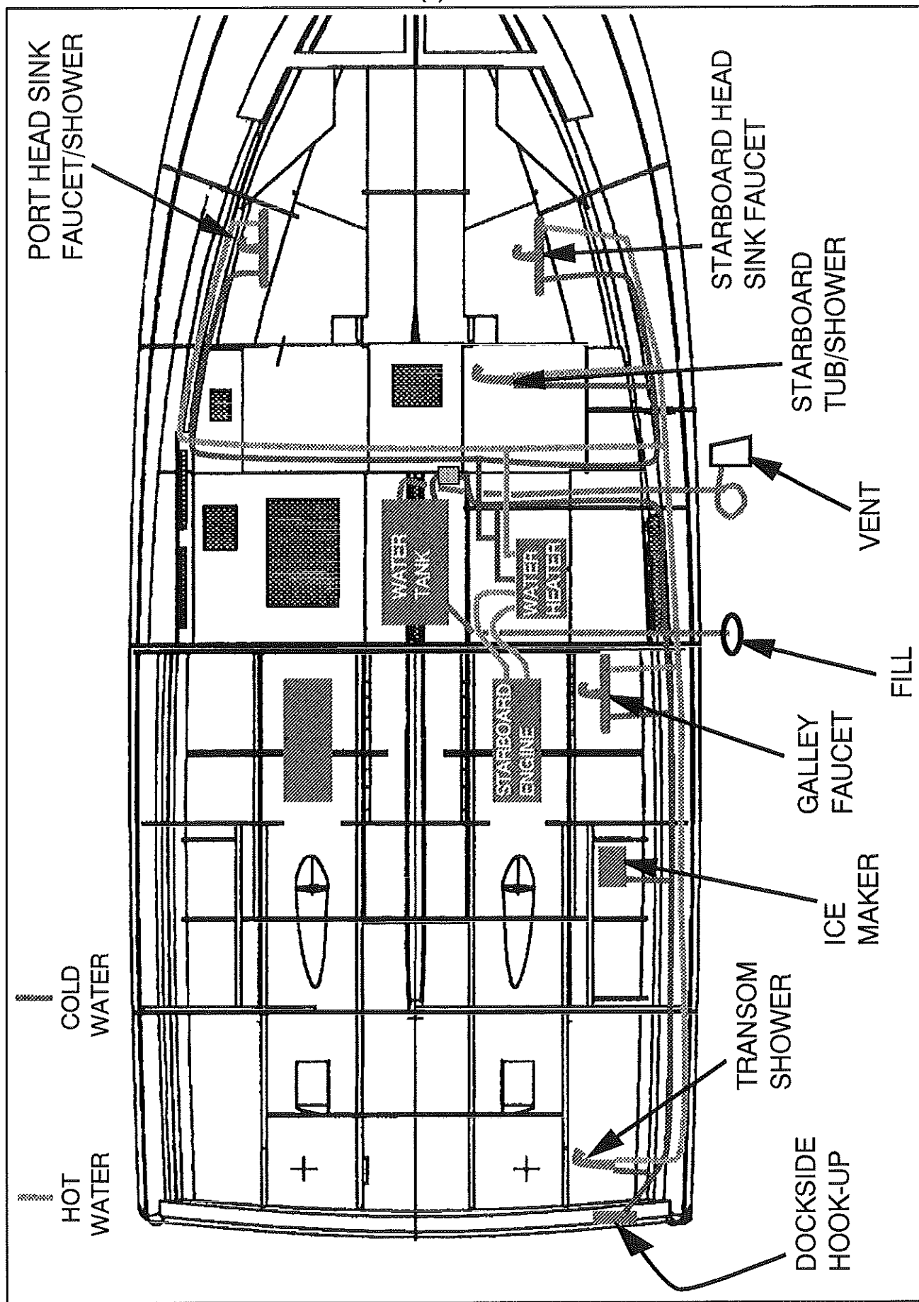
POTABLE WATER SYSTEM DIAGRAM (2)
