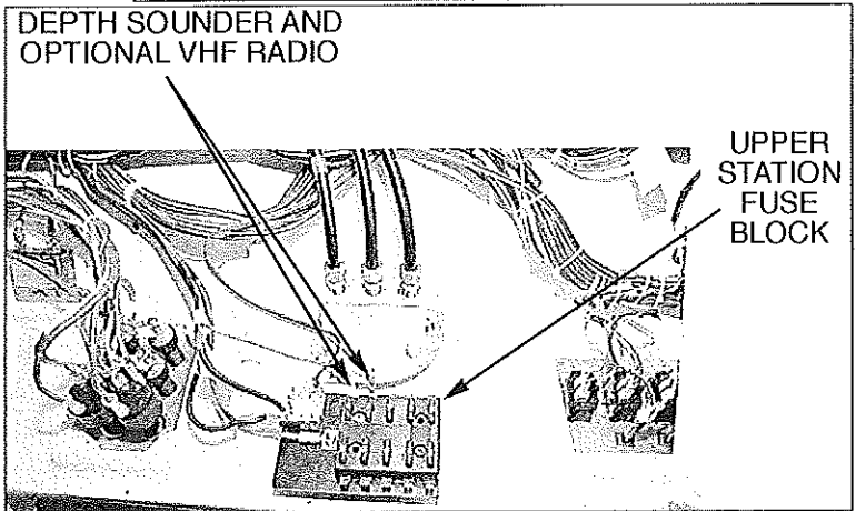
UPPER STATION FUSE BLOCK LOCATED ON UNDERSIDE OF DASH
